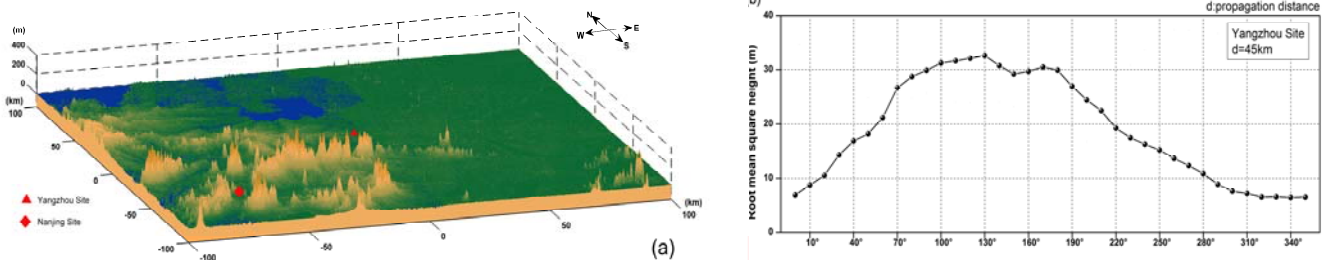
Fig. 1(a) Real irregular terrain map covering 200 \times 200 square kilometers around the Yangzhou DF site in Jiangsu province of China and (b) depicts the root-mean-squared height (RMSH) from the azimuth 0^\circ to 360^\circ .
