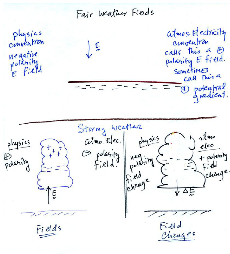
Fig. An early sketch used to illustrate the ‘Atmospheric Electricity’ and ‘Physics’ sign conventions at the University of Arizona.
